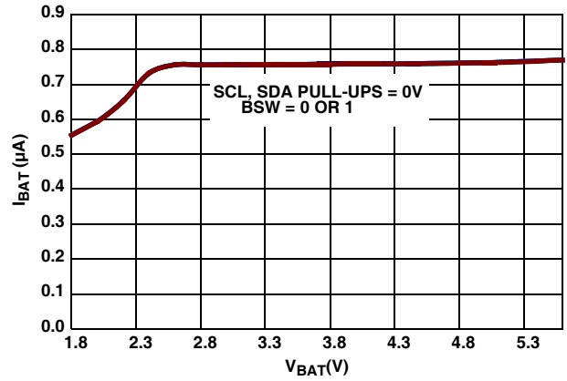
FIGURE 2. I_{BAT} vs V_{BAT} SBI3 = 1
