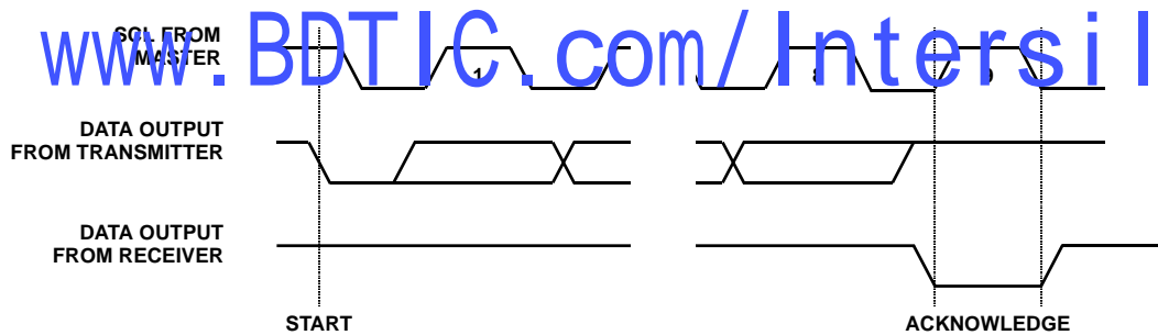
FIGURE 14. ACKNOWLEDGE RESPONSE FROM RECEIVER
