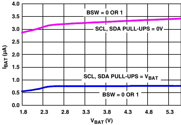
FIGURE 1. I_{BAT} vs V_{BAT} SBI3 = 0
