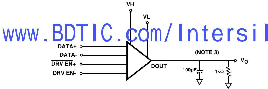
FIGURE 1. DRIVER SWITCHING TEST CIRCUIT
