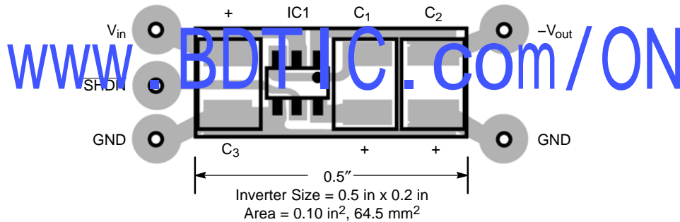
Figure 52. Inverter Circuit Board Layout, Top View Copper Side
