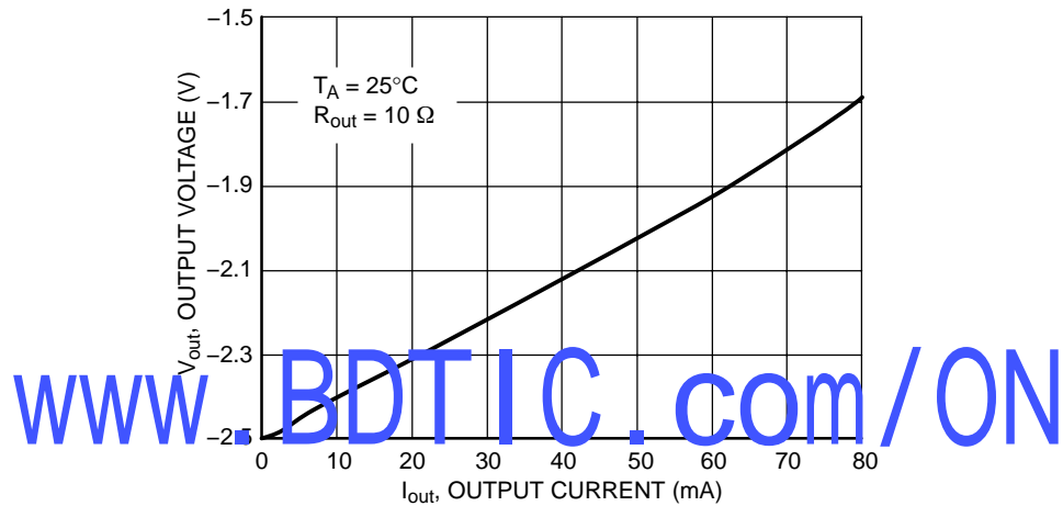
Figure 48. Negative Voltage Splitter Load Regulation, Output Voltage vs. Output Current
