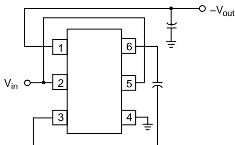
This device contains 77 active transistors. Figure 1. Typical Application
