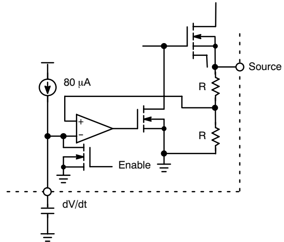
Figure 9. dV/dt Circuit
